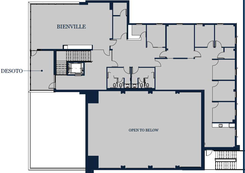
THE VALDRY CENTER FOR PHILANTHROPY SECOND FLOOR PLAN
